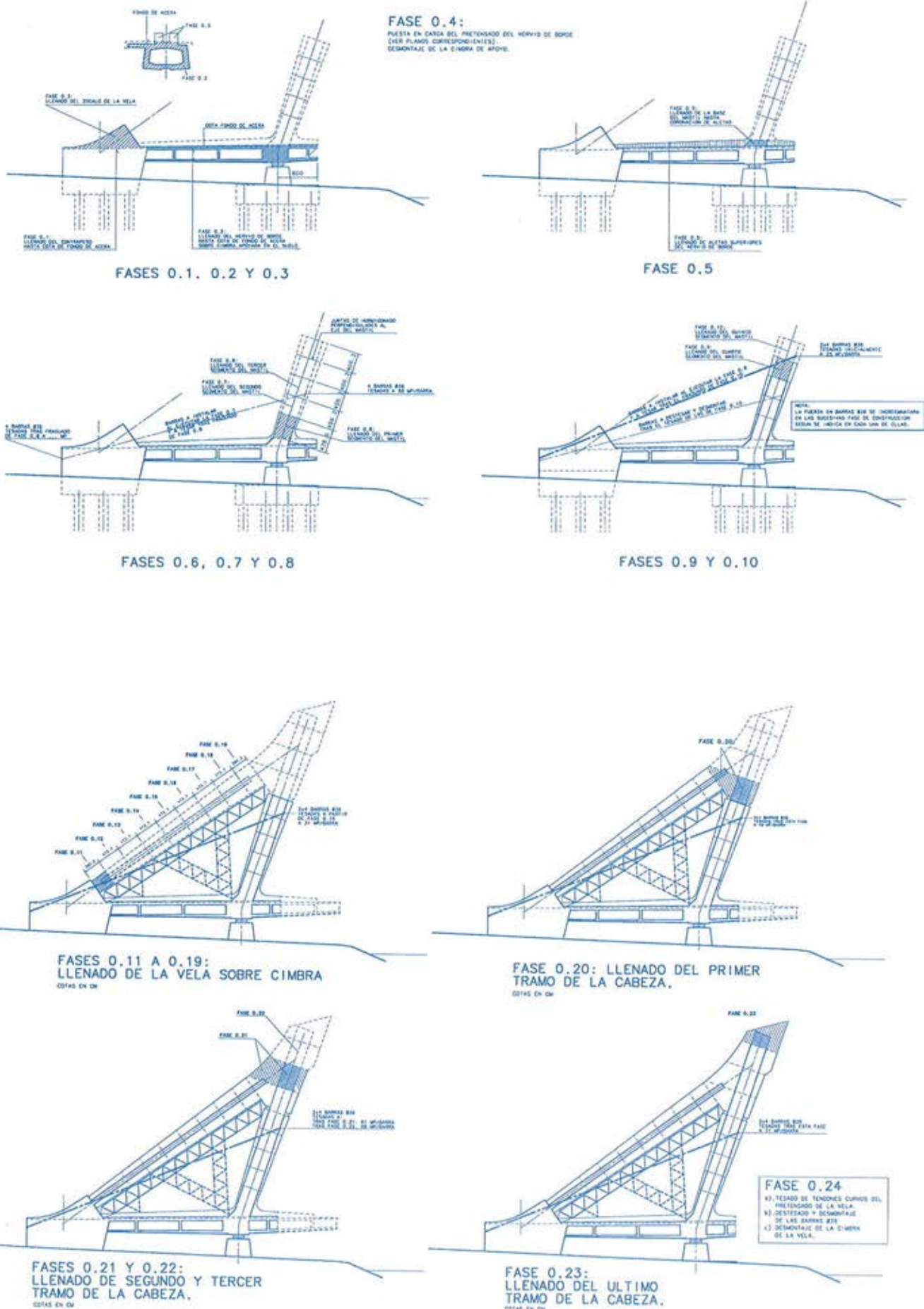
Figura 18: Proceso constructivo de las células laterales. Figure 18: Constructive Process of the Lateral Cells.
