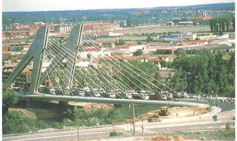
Figura 12. Vista del puente durante la prueba de carga. Figure 12. A view of the bridge during the loading test.
