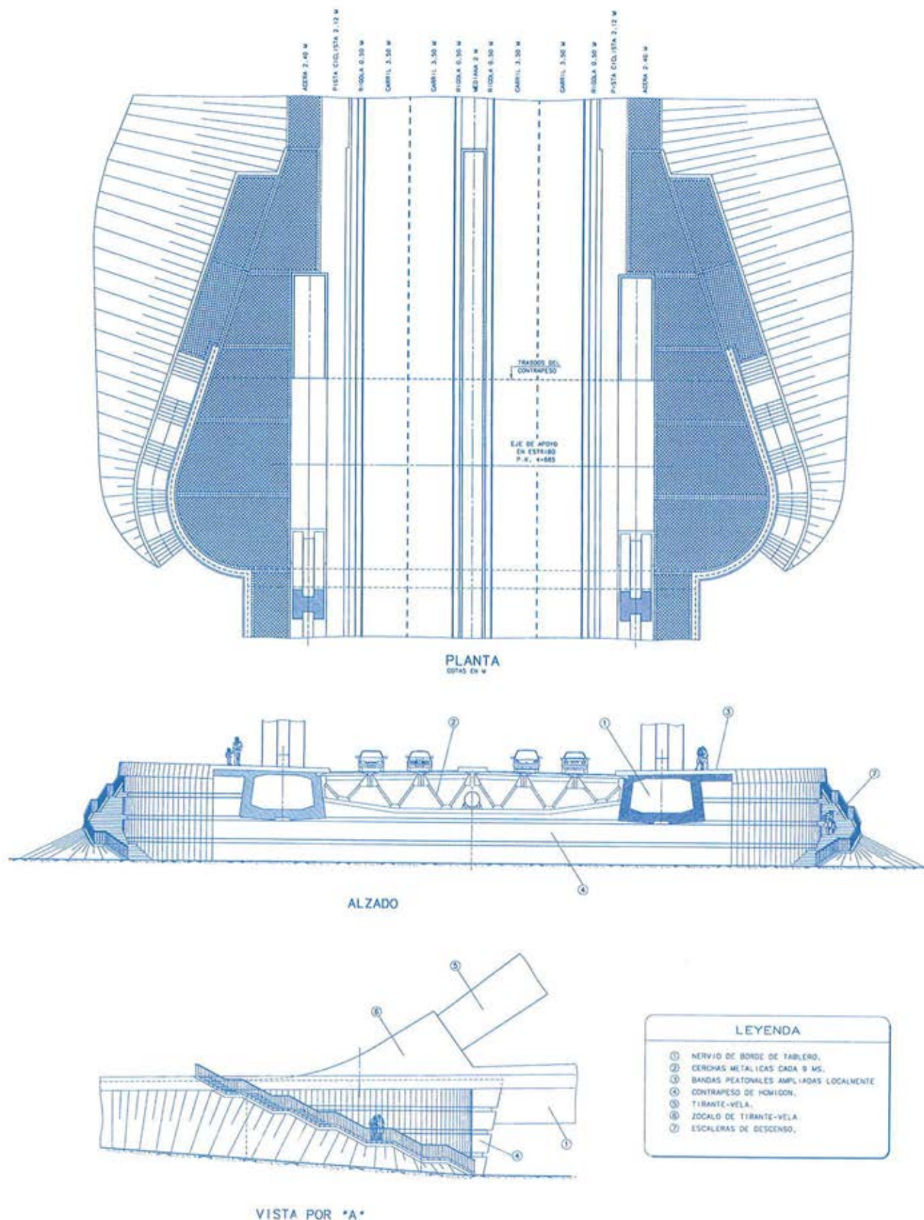
Figura 3: Planta, sección transversal y alzado del contrapeso final Figure 3: Plan, transverse cross-section and elevation of the concrete counterweight.
