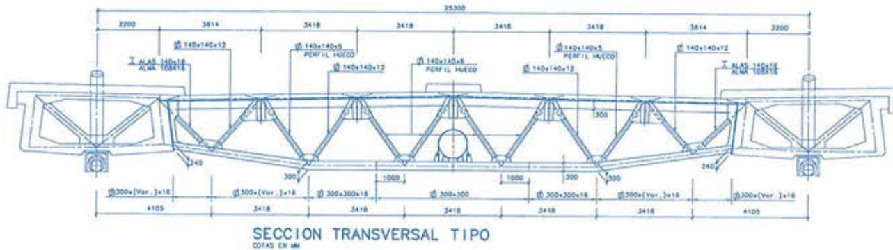
Figura 17: Geometría de cercha transversal. Figure 17: Geometry of the traverse trusses
