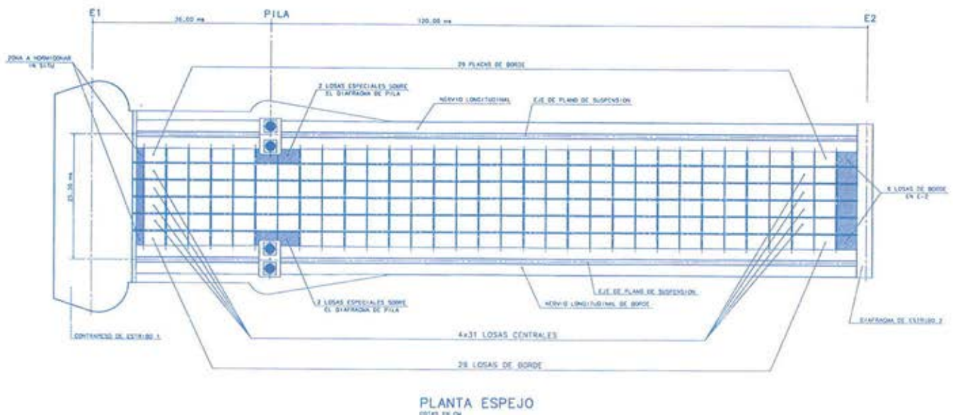
Figura 8: Planta espejo del tablero. Figure 8: Mirror plan of the deck.
